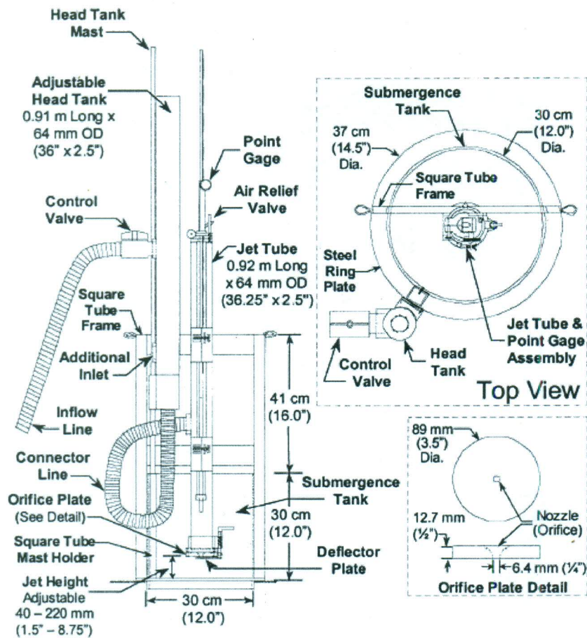
Figure 1 Schematic JET Apparatus
